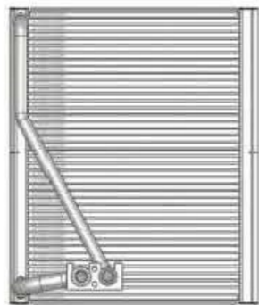
JLS-SC-054 MODEL:KIA RONDO 07-10 OEM:971401D000 SIZE:300x250x38
