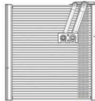
JLS-SC-105 MODEL: KIA CERATO 2012 FORTE SIZE: 265x278x34
