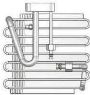
JLS-EV-056 MODEL: HONDA CRV 4 ROWS CIVIC 94-97 OEM: 80210 SRA12
