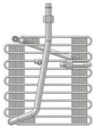
JLS-EV-088 MODEL:PATHFINDER 93-95 EAGLE OEM:2728058G05 SIZE:234x236x100
