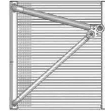
JLS-SC-029 MODEL: SIZE: 275x250x38
