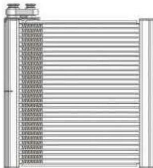
JLS-SC-096 MODEL: TOYOTA PICKUP SIZE: 223x225x48
