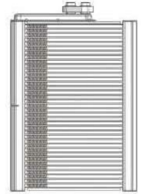
JLS-SC-126 MODEL: NISSAN SERENA C24 SIZE: 210x270x48
