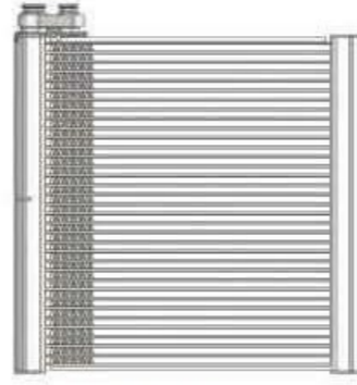
JLS-SC-262 MODEL: SIZE:255x250x48
