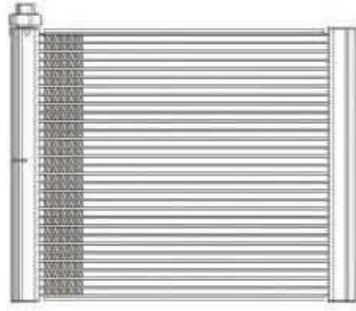
JLS-SC-040 MODEL:NISSAN SKYLINE SIZE:275x220x48
