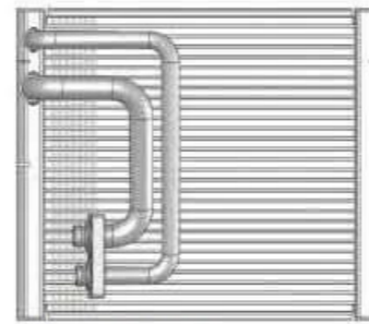
JLS-SC-102 MODEL: HYUNDAI HI GRAND STAREX REAR SIZE: 212x250x38
