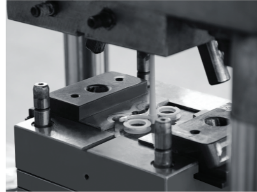
High-Precision mould
