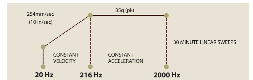
Figure 4: Vibration profile during vibration durability test
