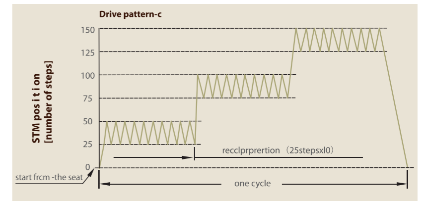
Figure 2 Move mode figure of DLA during vibration durability test and life cycling test
